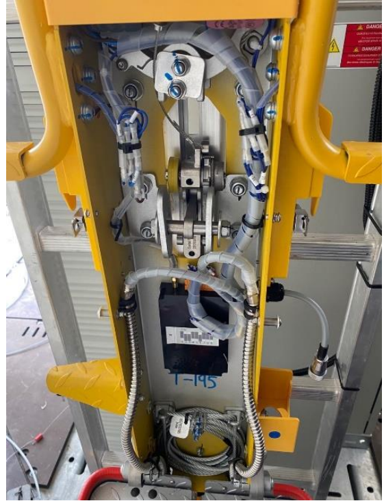
Traction Unit
